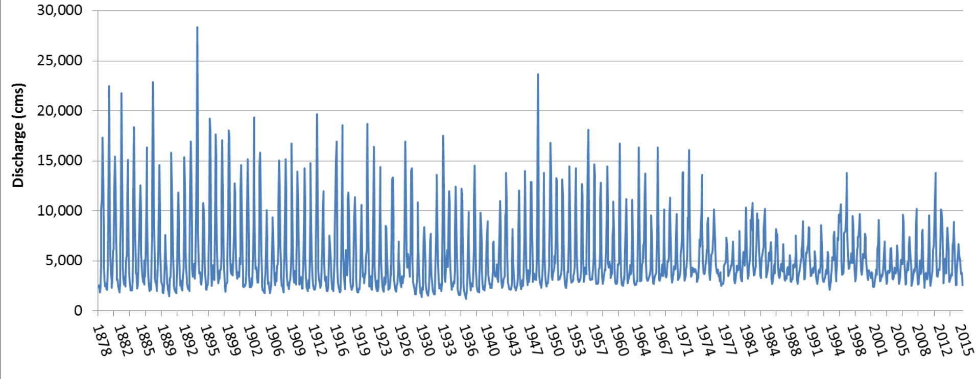
Average Monthly Discharge at The Dalles (rkm 310)
